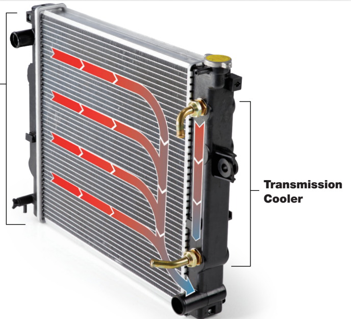
Engine Radiator
